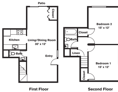
Townhome ~ Standard
