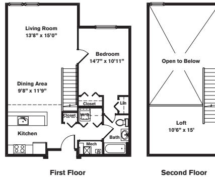
Two Floors
