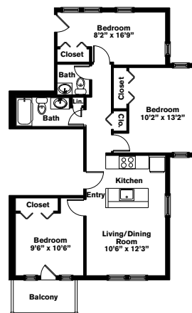
Three Bedrooms ~ 1.5 Baths (893 sq. ft.)
